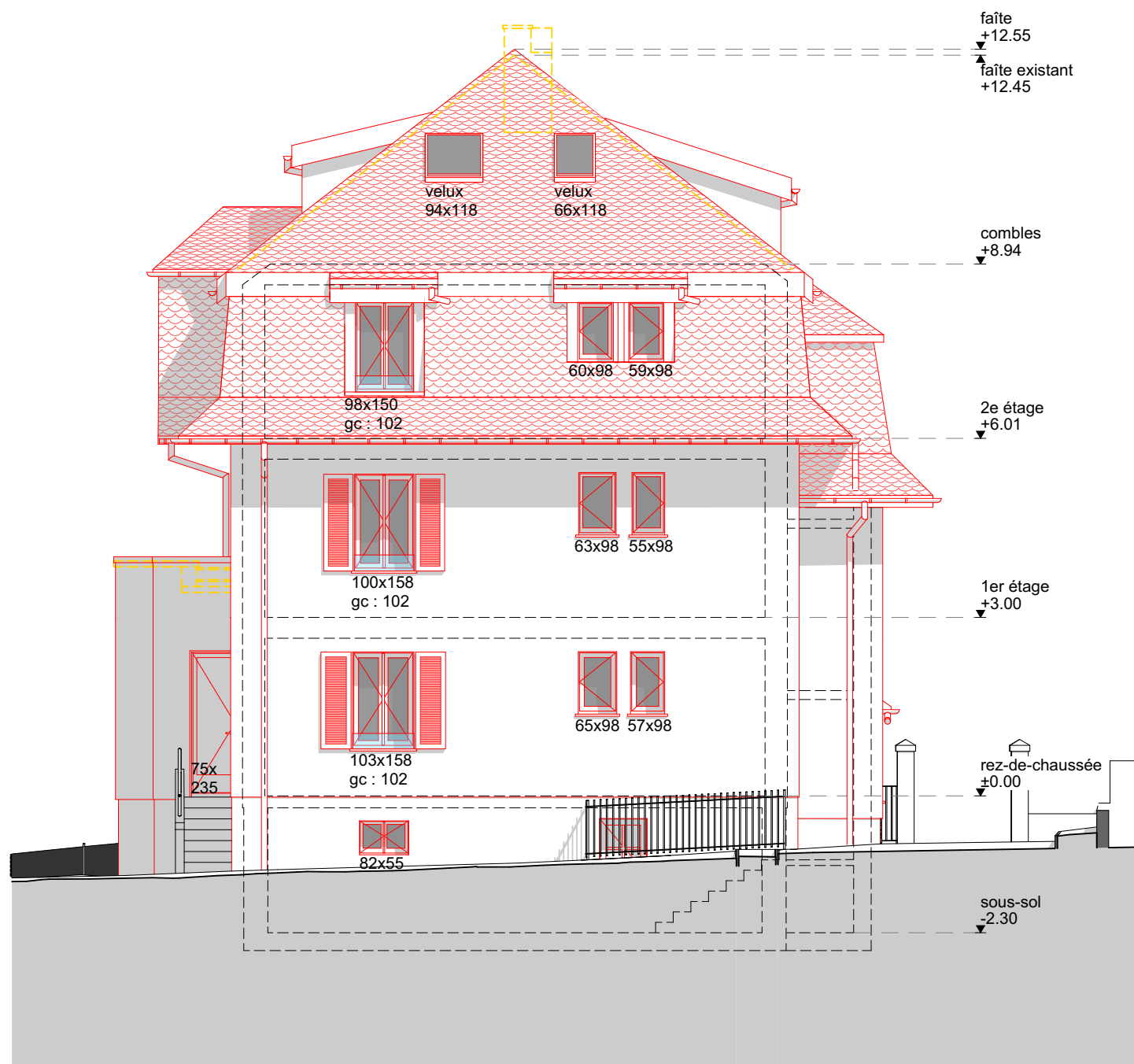
FACADE SUD
